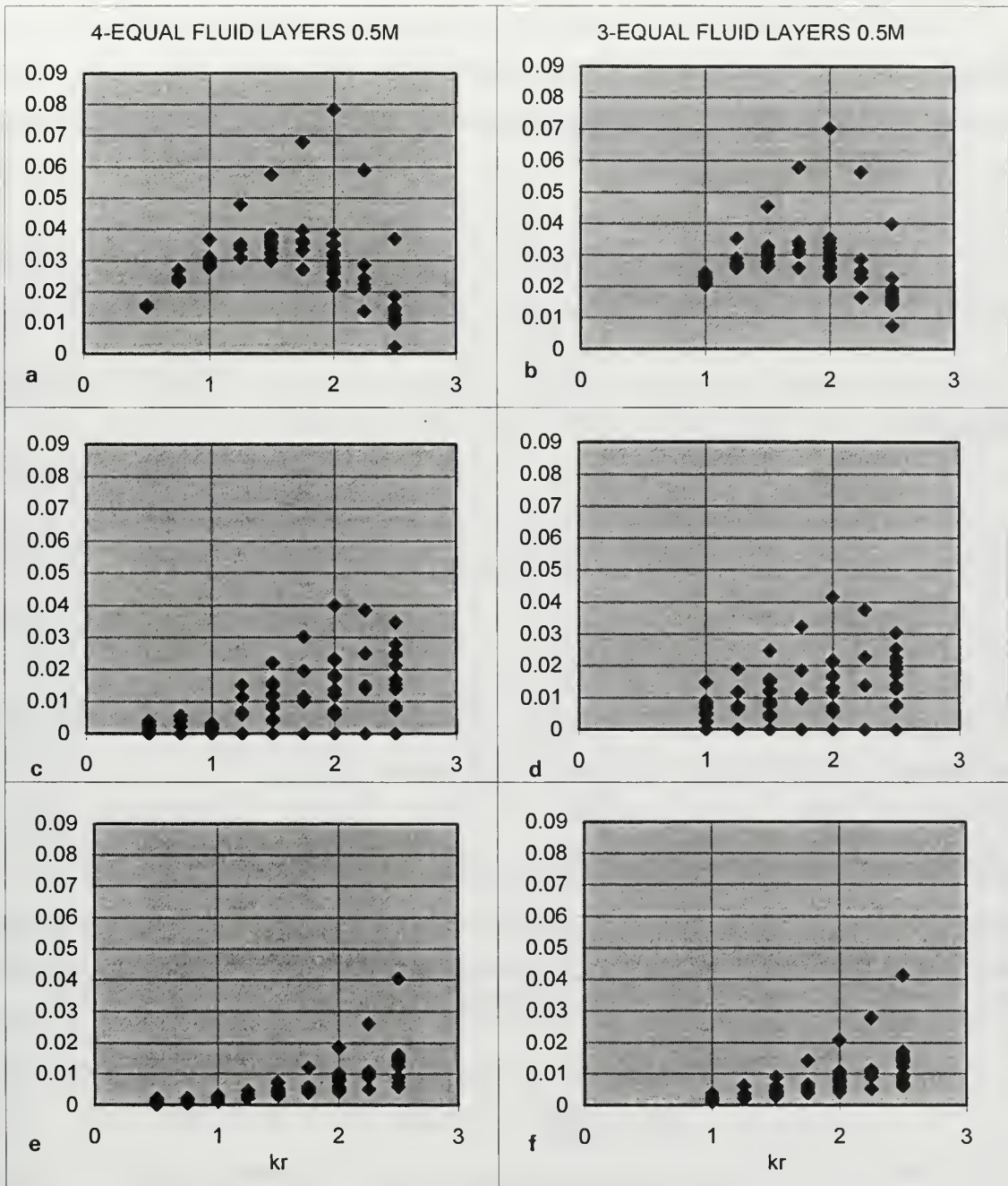
Figure 10. Normalized scattered pressure deviation computed by ATILA versus kr . From top to bottom monopolar (a,b), dipolar (c,d) and quadrupolar (e,f) incident field; on the left: scatterer radius ka = 0.5 ; on the right: scatterer radius ka = 1.0 , radiation boundary R and element size L satisfy: kR = 2.5 and kL = 0.5 for all cases.
